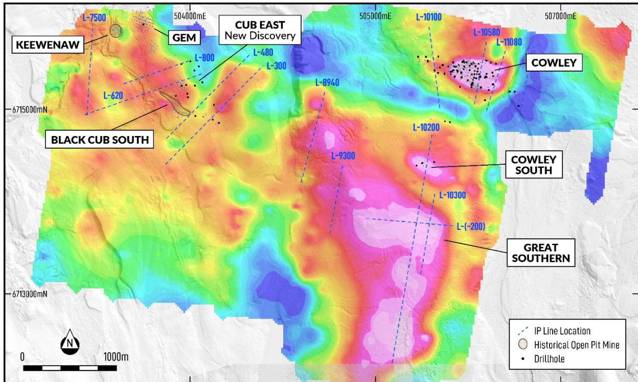
Figure 4: Plan map of Black Cub to Cowley over ground gravity, showing completed IP Lines.
