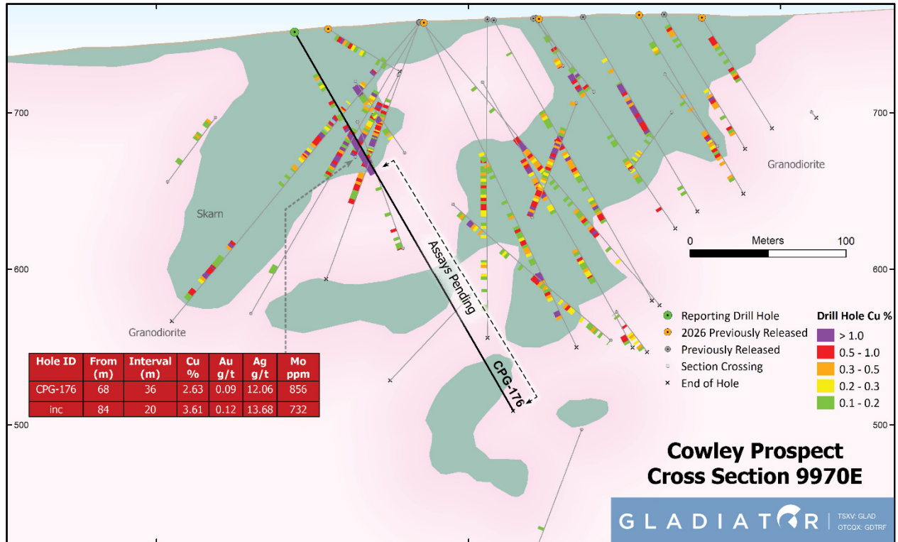
Figure 2: Section 9,970E through Cowley, viewed west, showing Gladiator drilling. New drill results reported in this release are highlighted in red. Refer to Figure 1 for the section location.
