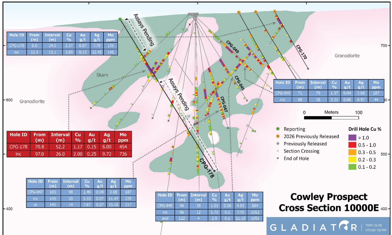
Figure 3: Section 10,000E through Cowley, viewed west, showing Gladiator drilling. New drill results reported in this release are highlighted in red. Refer to Figure 1 for the section location.
