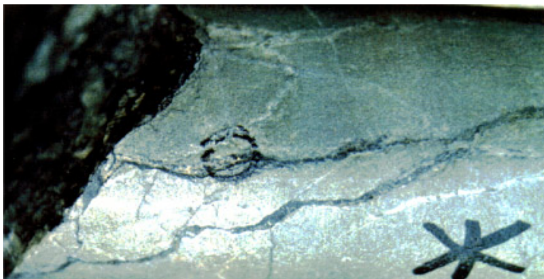
Plate 2. Photograph of drill core from MDD-001. Note presence of visible gold within a low amplitude, black graphite-chlorite-pyrite stylolite seam, within sericite altered, hydrofractured sandstone. (Assay 75-76m: 12.0 g/t Au).
